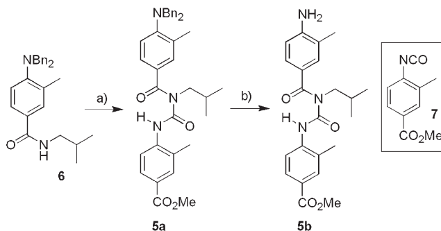
Scheme 1. Synthesis of 5b . Reagents and conditions: a) LiHMDS, THF, –78 °C, 5 min, then 7 , –78 °C, 15 min; b) H 2 , Pd/C, EtOAc/MeOH. Bn = benzyl, HMDS = hexamethyldisilazide.
